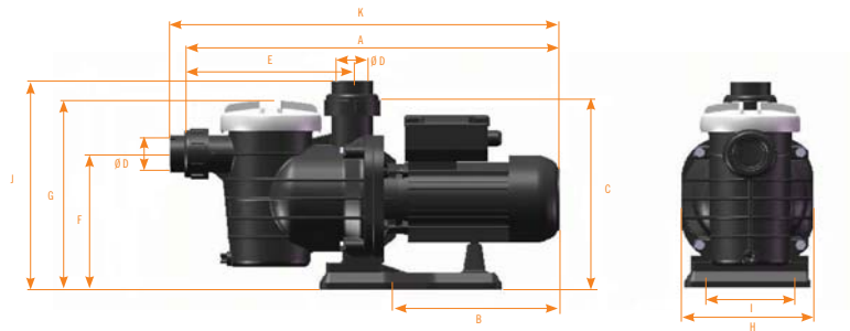
Dimensiones bombas Alaska Alaska Pump dimensions
