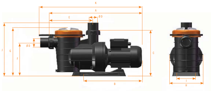
Dimensiones bombas Alaska Max Alaska Max Pump dimensions
