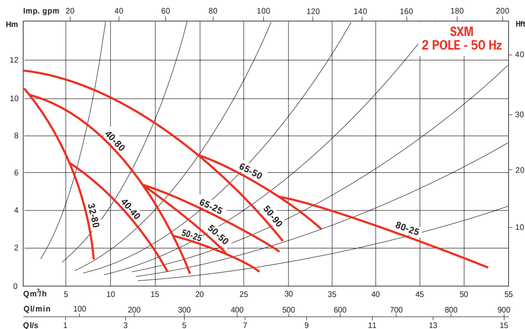
SXM - Single Circulator 2 POLE - 1-PHASE 50 Hz
