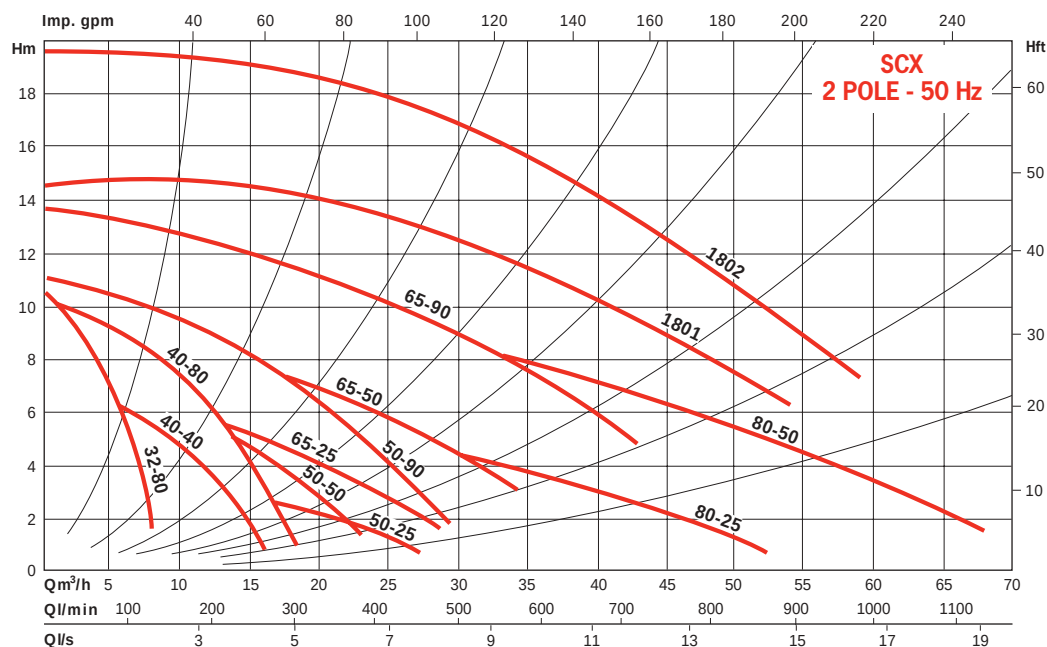
SCX - Single Circulator 2 POLE - 3-PHASE 50 Hz
